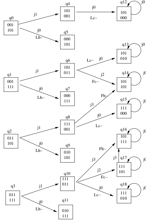
Figure 2. Developments from the four possible initial states.
