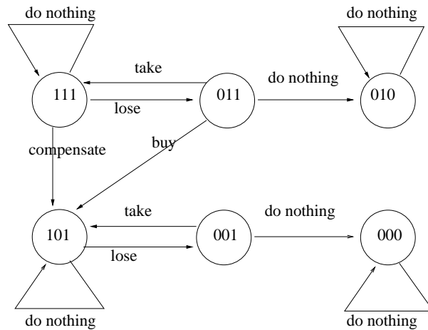
Figure 1. State transition diagram for our agents
