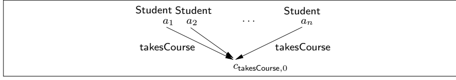
Fig. 3. Canonical model \mathcal{I}_{\mathcal{K}} for Example 6.
