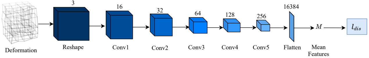
Fig. 4. The structure of the discriminator D_\theta used in the Discrimination Loss ( I_{dis} ) of our Adversarial Learning with Distilling Knowledge algorithm.
