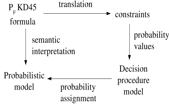
Fig. 2. Relation between P_FKD45 and decision procedure.
