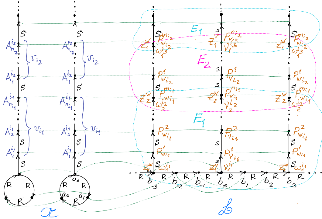
Figure 1: Intended models \mathfrak{A}, a_0 and \mathfrak{B}, b_0 with \mathfrak{A} \models \varphi(a_0) , \mathfrak{B} \models \neg\psi(b_0) , and \mathfrak{A}, a_0 \sim_{L, \varrho} \mathfrak{B}, b_0 , where \varrho -bisimilar points in the disjoint union of \mathfrak{A} and \mathfrak{B} are connected by dotted lines and E_i -equivalence classes in \mathfrak{B} , i = 1, 2 , are encircled by dashed lines. Model \mathfrak{A} contains two disjoint copies of a 3-point R -cycle followed by an infinite S -chain. Model \mathfrak{B} has an infinite R -chain of points b_i , for i \in \mathbb{Z} ; each b_{6i} starts an infinite S -chain for the word v_{i_1} v_{i_2} \dots , and each b_{6i+3} starts an infinite S -chain for the word w_{i_1} w_{i_2} \dots . These \omega -words coincide with the \omega -word written on the S -chains in \mathfrak{A} .
