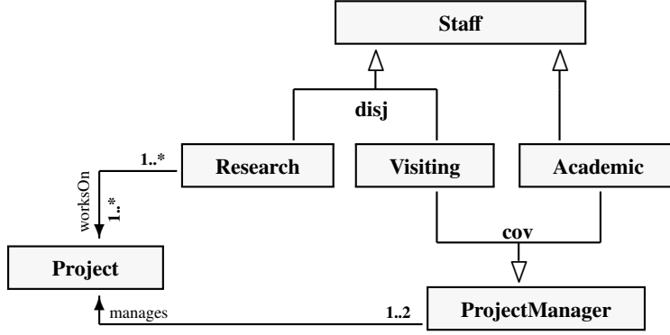
Figure 1: A UML class diagram.
