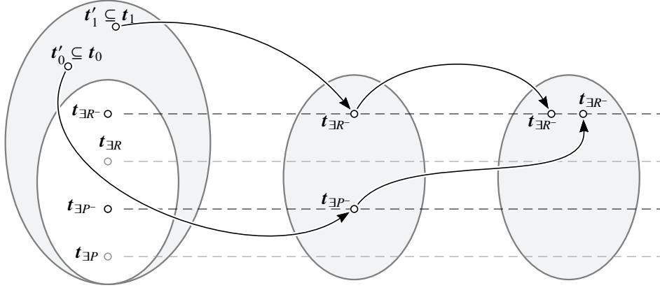
Figure 2: The first three steps of constructing a model realising \{t'_0, t'_1\} by means of unravelling.
