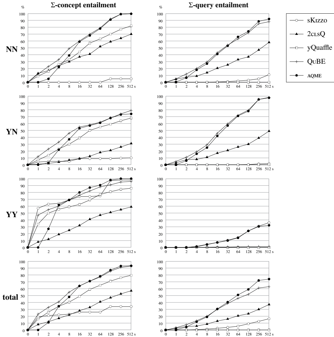
Figure 4: Percentage of solved instances.
