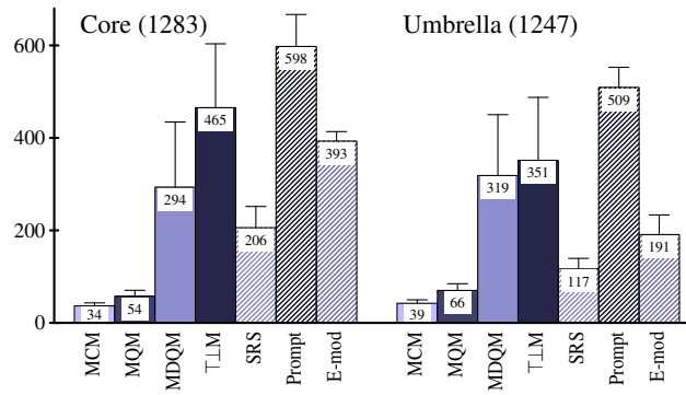
Figure 5: Module sizes for |\Sigma| = 10 and standard deviation.
