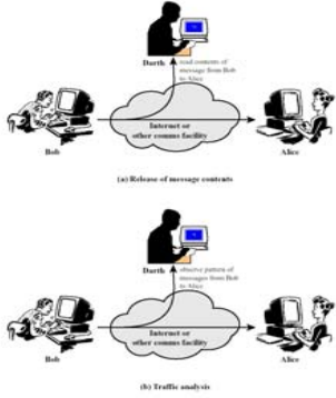
Figure 1.1 Passive Attacks
