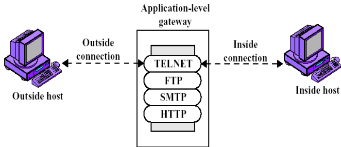
(b) Application-level gateway
