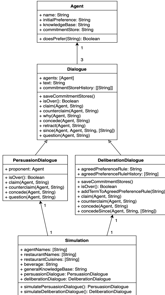
Fig. 1. Class diagram
