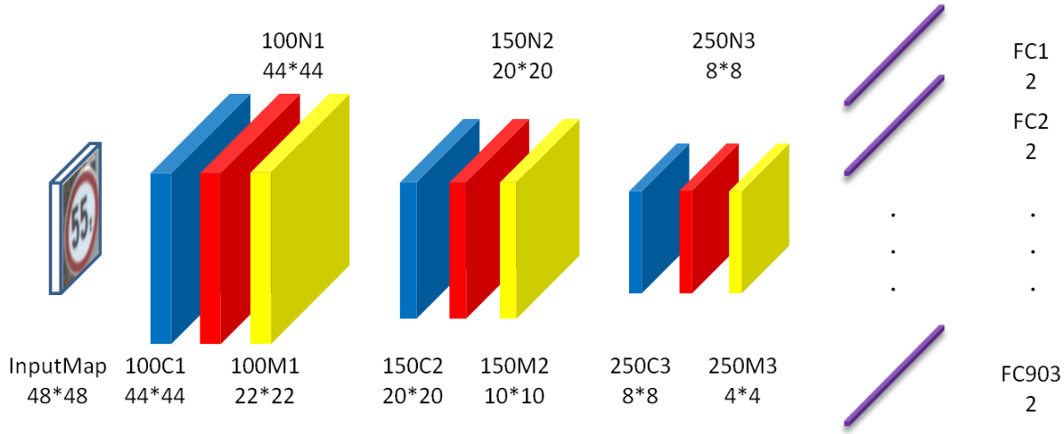
Fig. 3. Network architecture in testing stage
