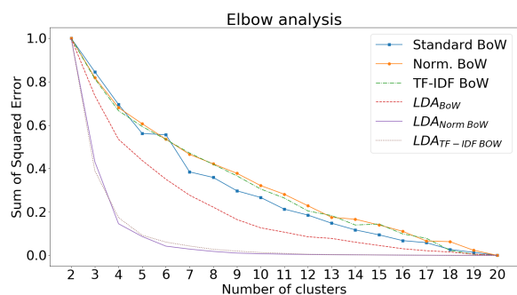
Figure (1) Elbow analysis of the Unspecified Label Pagination approach.
